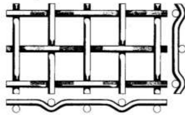
Flat top Crimp
